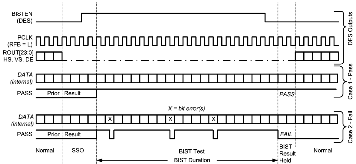
FIGURE 16. BIST Waveforms
