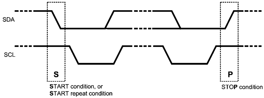
FIGURE 18. START and STOP Conditions
