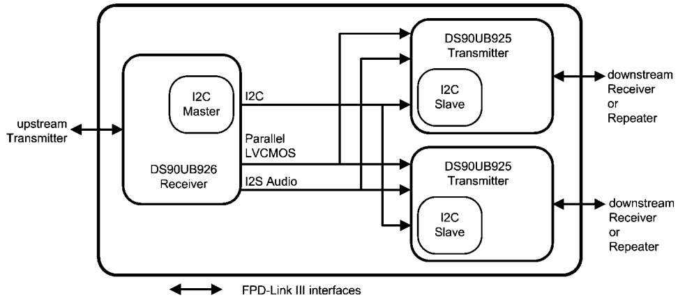
FIGURE 13. 1:2 Repeater Configuration
