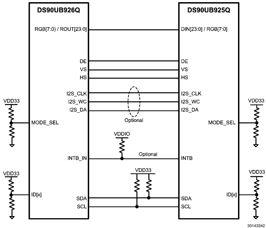
FIGURE 14. Repeater Connection Diagram
